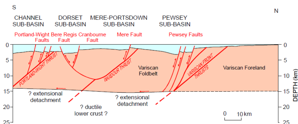
Figure 16. Crustal section across the Wessex and western Weald basins, illustrating the influence of extensional reactivation of Variscan thrusts (after Chadwick 1986). See Figure 18 for location.
