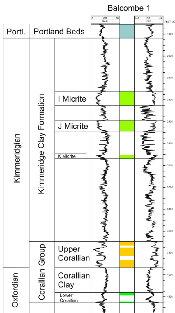
Figure 25. The Kimmeridge Clay and associated micrites in Balcombe 1. Note the maximum gamma-log response of only 100 API.
