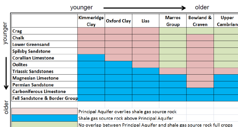
Figure 8. The stratigraphic relationship between principal aquifers and shale source rocks in England (from Bloomfield et al. 2014).
