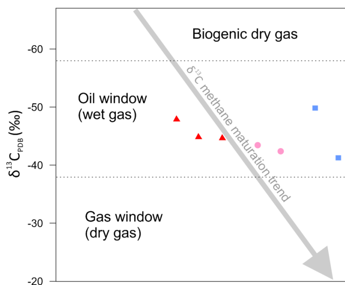
Figure 40. Maturation trend of \delta^{13}\text{C} methane through the oil and gas windows (Stahl 1977) and \delta^{13}\text{C} methane of the Weald Basin gas samples (from Conoco 1986).
