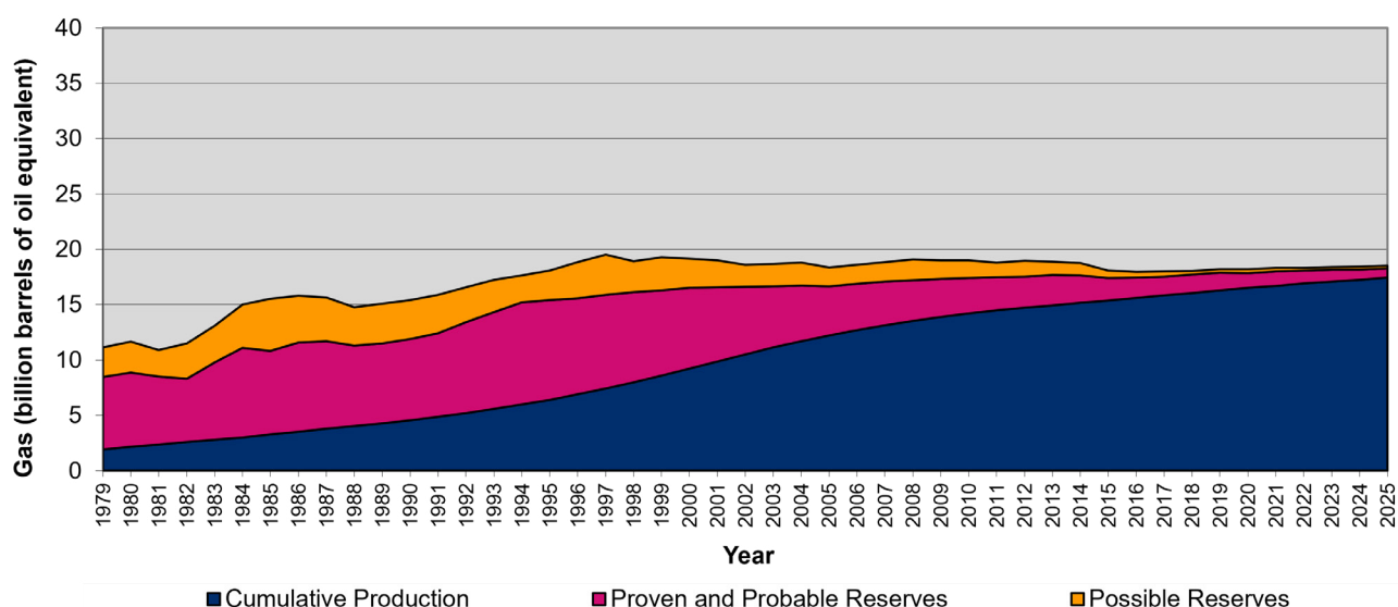
Figure 7: Gas Estimated Ultimate Recovery vs time (to end 2025)
