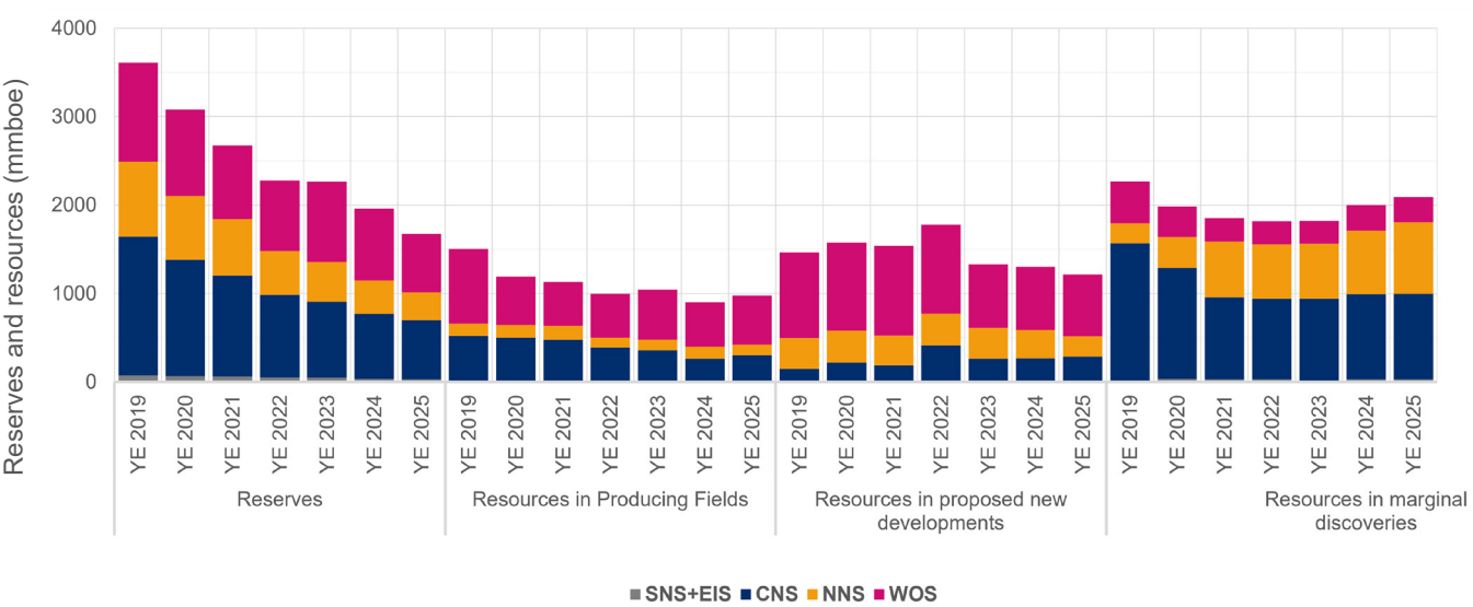
Figure 9: Oil reserves and resources by area (2P/2C)
